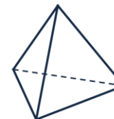
Tetraedrul regulat
