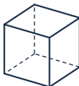
Cubul
